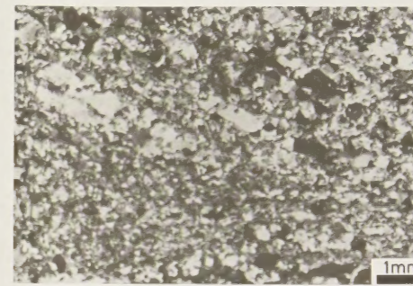
Figure 8. The fine-grained, strongly recrystallized quartz-feldspar-rich mylonitic fabric of the rock is illustrated in the photomicrograph above, viewed parallel to the mineral lineation in the rock. The S 2 schistosity is outlined by elongate quartz ribbons (upper left to lower right). Note the banding of these ribbons (center). Sericite is common, but typically not abundant, suggesting that chemical alteration of feldspar was not extensive.
